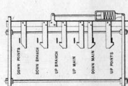
PLAN VIEWS. - LEVERS IN SECTION.
