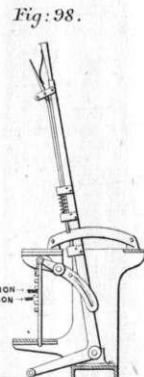
CROSS ELEVATION. FRONT ELEVATION. EASTERBROOKS' RECENT GEAR.
