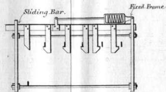
PLAN VIEWS. - LEVERS IN SECTION.
