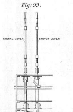
CROSS ELEVATION. FRONT ELEVATION. EASTERBROOKS' RECENT GEAR.
