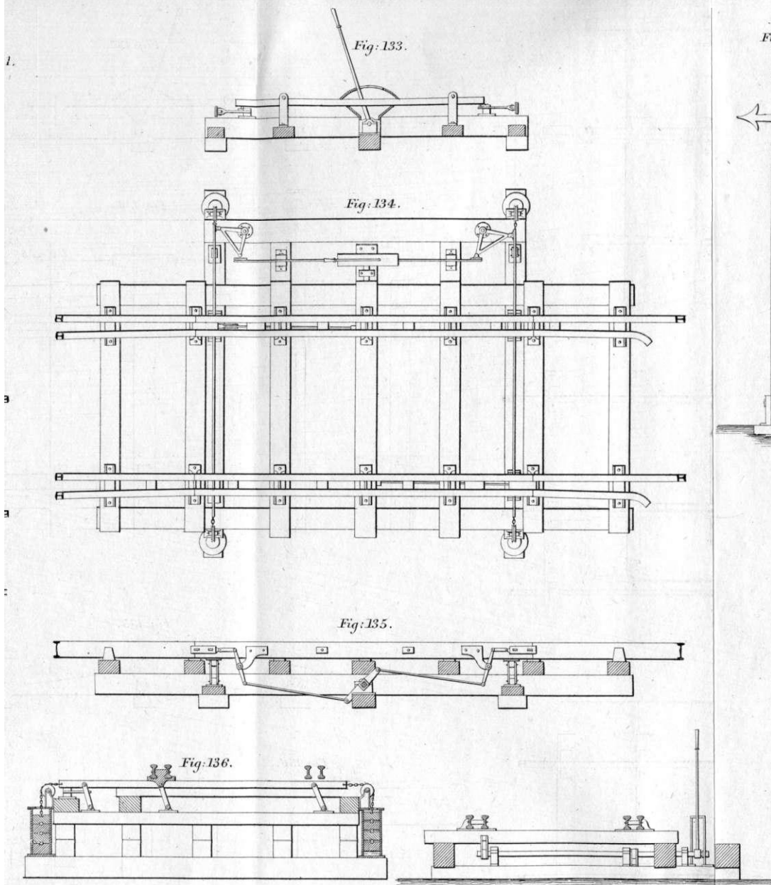
MR. R. PRICE WILLIAMS' SWITCHES.
