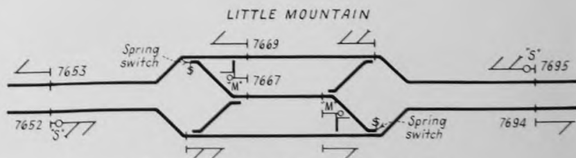
Fig. 4—Track and signal plan of Little Mountain
