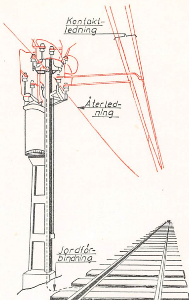
Fig 3 Sugtransformatorstolpe
